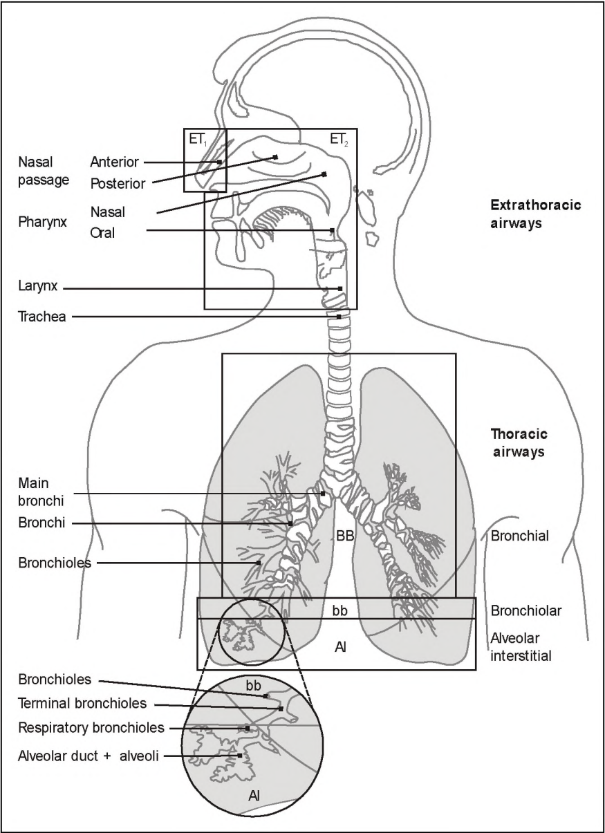
FIGURE 9 Respiratory tract regions defined in the HRTM (based on ICRP, 1994)
