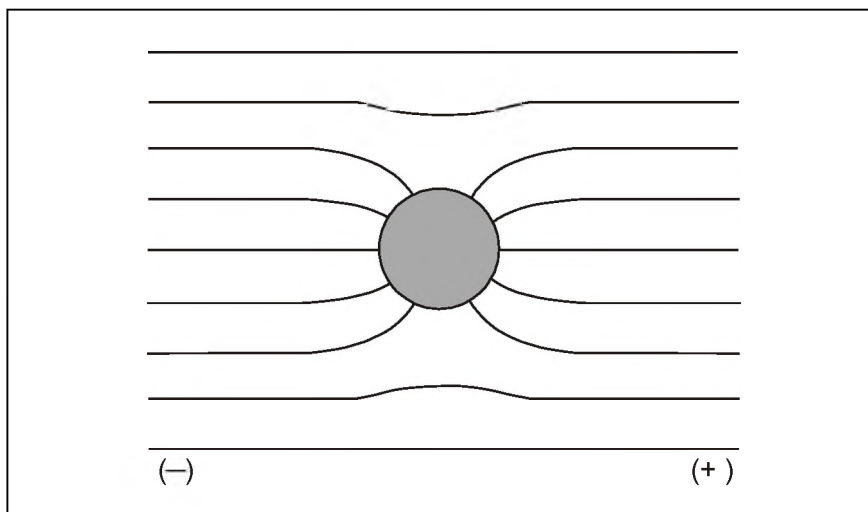
FIGURE 6 Distorted electric field around a spherical particle
