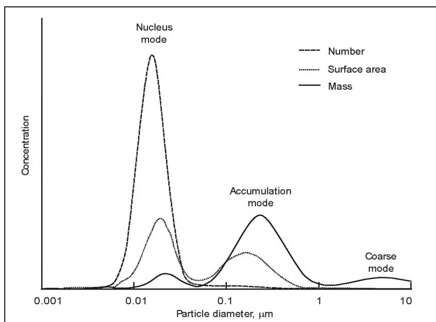
FIGURE 1 Size distributions of airborne particles by number, surface area, and mass (the diagram is illustrative; real distributions depend strongly on location and vary with time – see text)
