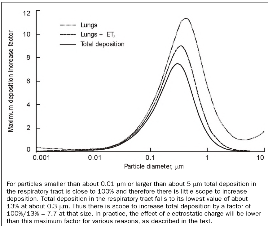
FIGURE 12 Scope for increasing deposition of unit density spheres in the respiratory tract (deposition conditions and combinations of regions as in Figure 11)
