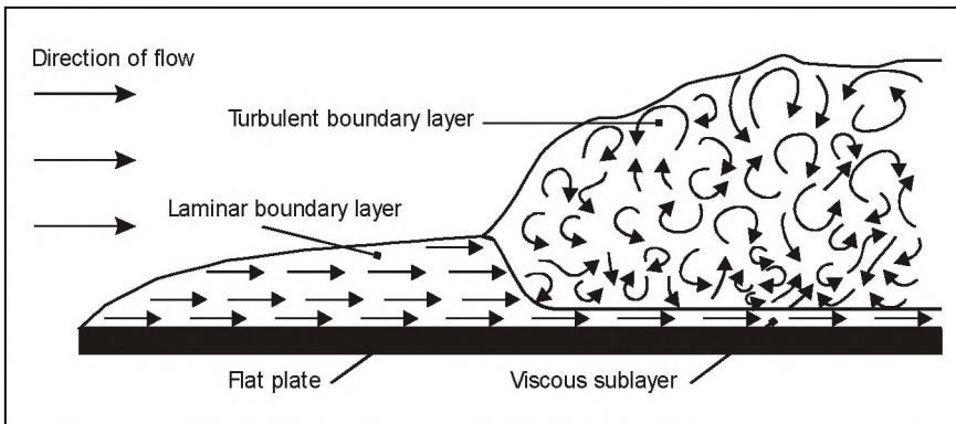
FIGURE 13 Laminar and turbulent flow across a flat plate
