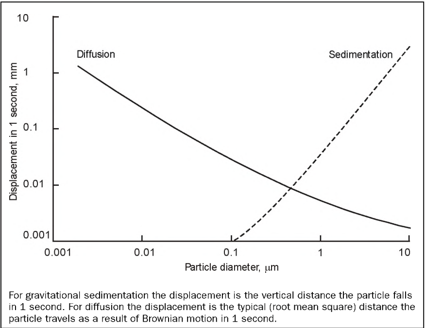
FIGURE 3 Relative importance of gravitational sedimentation and diffusion as a function of particle size (for unit density spheres, data taken from Raabe, 1994)
