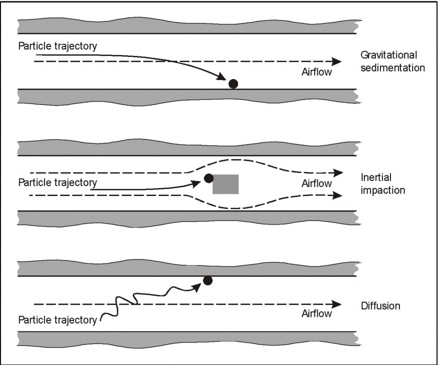
FIGURE 2 Main mechanisms of particle deposition
