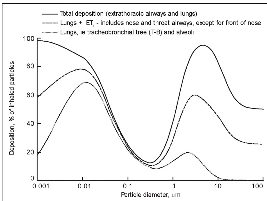
FIGURE 11 Particle deposition in the respiratory tract for unit density spheres inhaled by an adult male averaged over 24 hours, calculated using the HRTM
