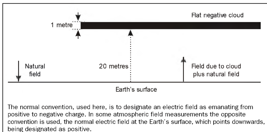
FIGURE 5 Effect of a cloud of charge on the Earth's field
