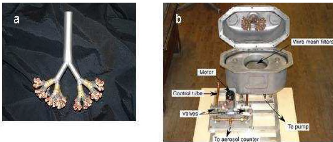
Model lung a) Showing the branching of the bronchial tree b) Showing the complete set-up
