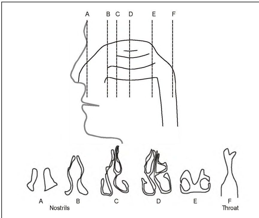
FIGURE 8 Cross-sections through the nasal passage (based on Häußermann et al. in press)
