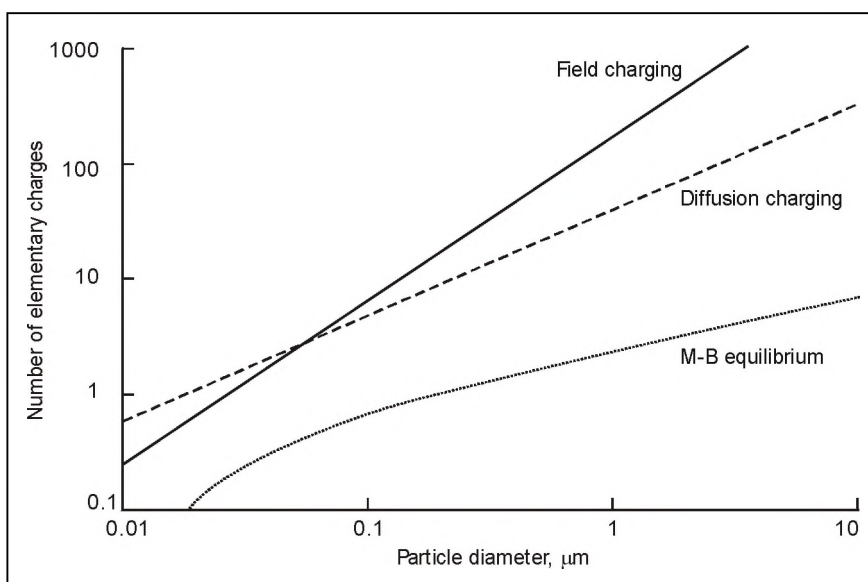
FIGURE 7 Limiting values of charge for different charging processes
