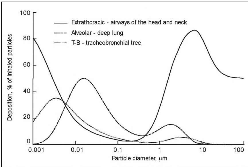
FIGURE 10 Particle deposition in the respiratory tract for unit density spheres inhaled by an adult male averaged over 24 hours, calculated using the HRTM
