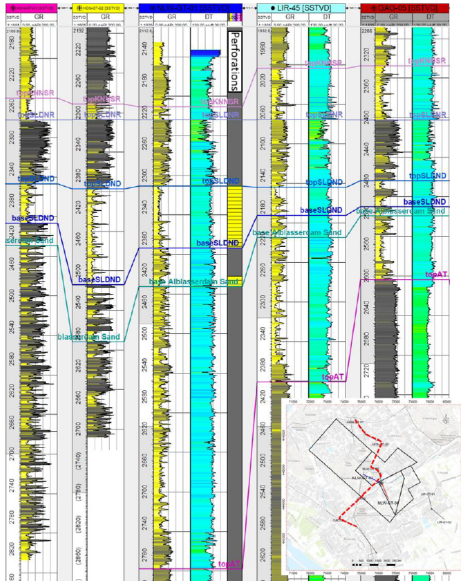
Figure 7-1: Regional correlation panel showing the gamma ray logs (non-normalised) flattened with respect to the top Rodenrijs Member (the inset map shows the location of the wells used, connected by the red, dashed line).
