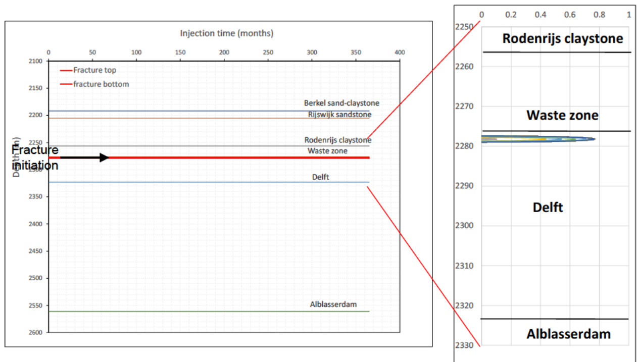
Figure 6-9: Fracture top and bottom as a function of time for base case; fracture contours for sensitivity 4. Fracture with 0.8 m radius which remains entirely in the Delft formation. BHIP = 0.232 bar/m.
