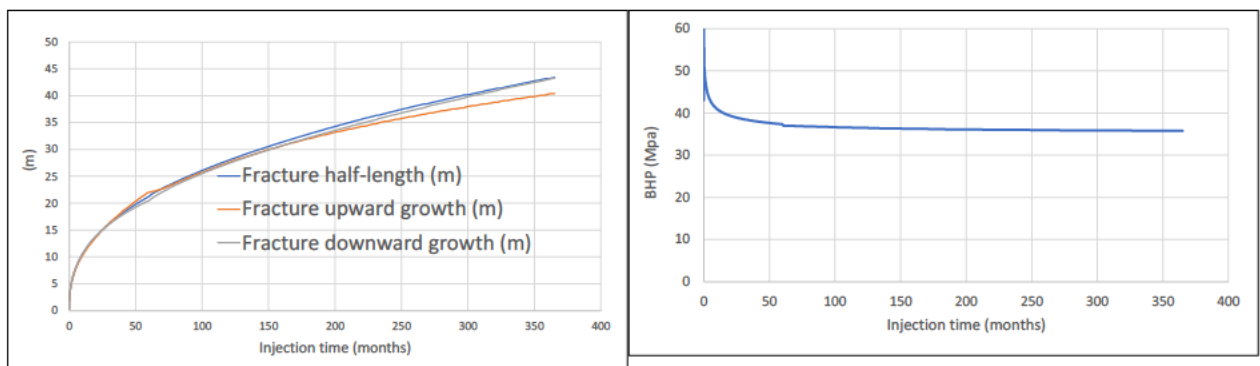
Figure 6-6: Fracture length, upward height, downward height, and Bottom Hole Injection Pressure (BHIP) for sensitivity 2. Fracture of 45 m radius after 30 years of injection, penetrating into water zone and overlying Rodenrijs shale. BHIP = 0.157 bar/m.
