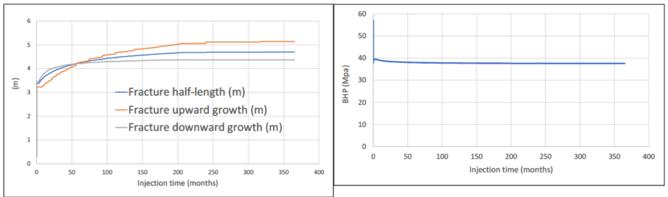
Figure 6-4 Fracture length, upward height, downward height, and Bottom Hole Injection Pressure (BHIP) for sensitivity 1. Fracture remains small (5 m), it penetrates 3 m into the waste zone. BHIP = 0.165 bar/m.
