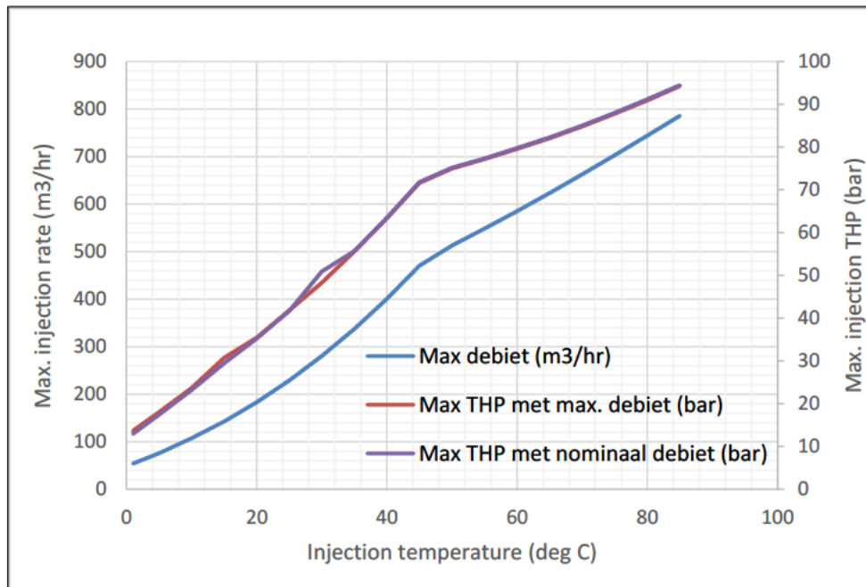
Figure 2-1: Maximum allowable injection rate and THP without allowing thermal fracturing for Polanen Delft formation, as a function of THT.
