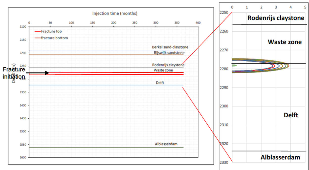
Figure 6-13: Fracture top and bottom as a function of time for base case; fracture contours for sensitivity 6. Fracture with 4 m radius and 2 m penetration into the waste zone. BHIP = 0.150 bar/m.
