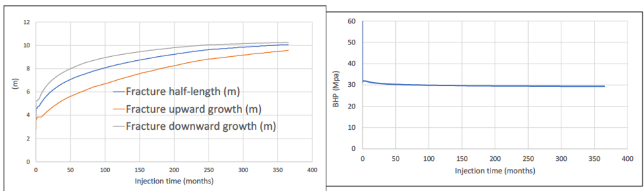
Figure 6-10: Fracture length, upward height, downward height, and Bottom Hole Injection Pressure (BHIP) for sensitivity 4. . Fracture with 0.8 m radius which remains entirely in the Delft formation. BHIP = 0.232 bar/m.
