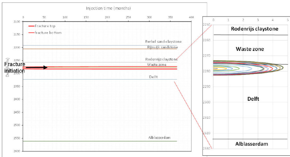
Figure 6-3: Fracture top and bottom as a function of time for base case; fracture contours for sensitivity 1. Fracture remains small (5 m), it penetrates 3 m into the waste zone. BHIP = 0.165 bar/m.
