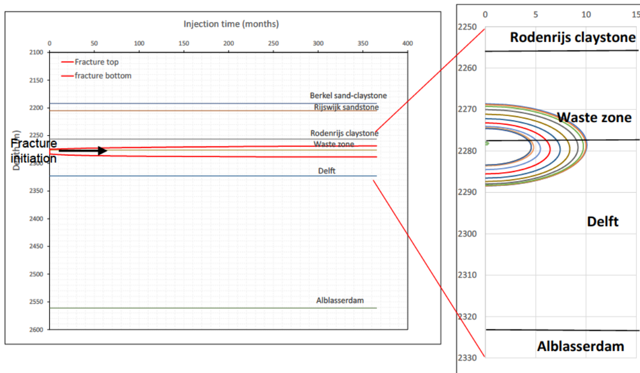
Figure 6-7: Fracture top and bottom as a function of time for base case; fracture contours for sensitivity 3. Fracture with 10 m radius and 8 m penetration into the waste zone. BHIP = 0.129 bar/m.
