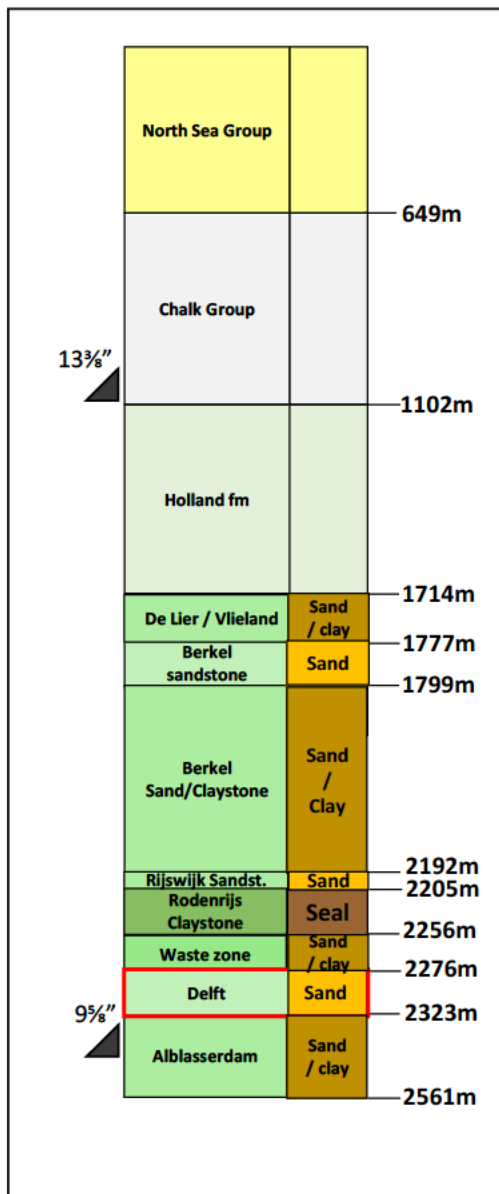
Figure 5-1: Stratigraphic scheme.
