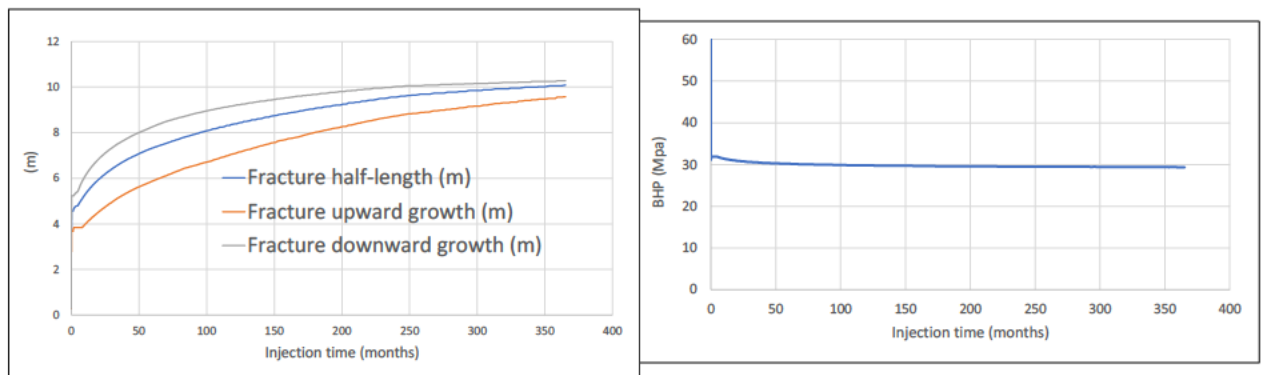
Figure 6-14: Fracture length, upward height, downward height, and Bottom Hole Injection Pressure (BHIP) for sensitivity 6. Fracture with 4 m radius and 2 m penetration into the waste zone. BHIP = 0.150 bar/m.
