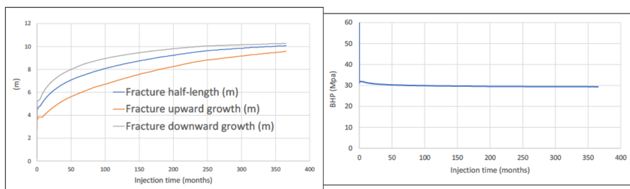
Figure 6-8: Fracture length, upward height, downward height, and Bottom Hole Injection Pressure (BHIP) for sensitivity 3. . Fracture with 10 m radius and 8 m penetration into the waste zone. BHIP = 0.129 bar/m.
