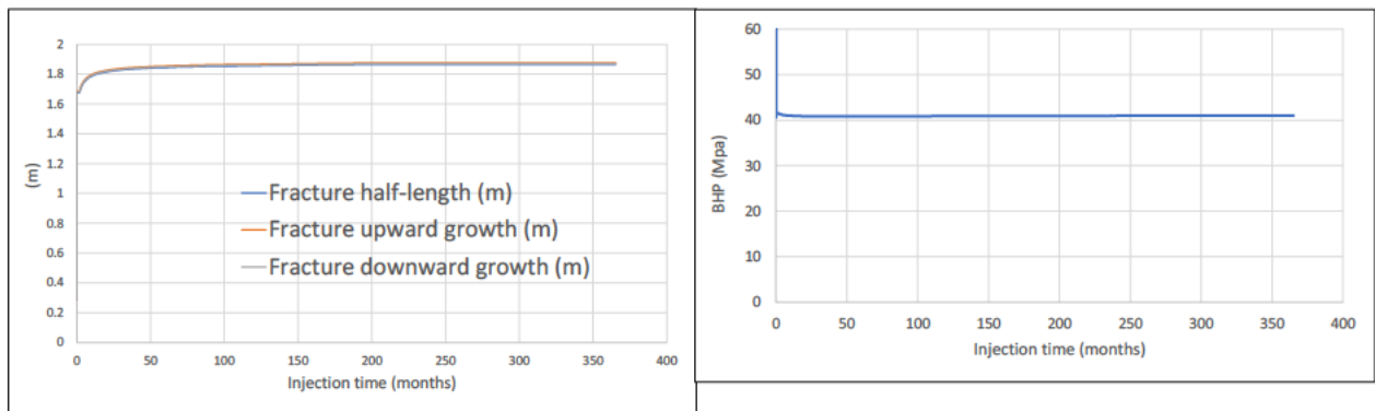
Figure 6-2: Fracture length, upward height, downward height, and injection Bottom Hole Pressure (BHP) for base case.
