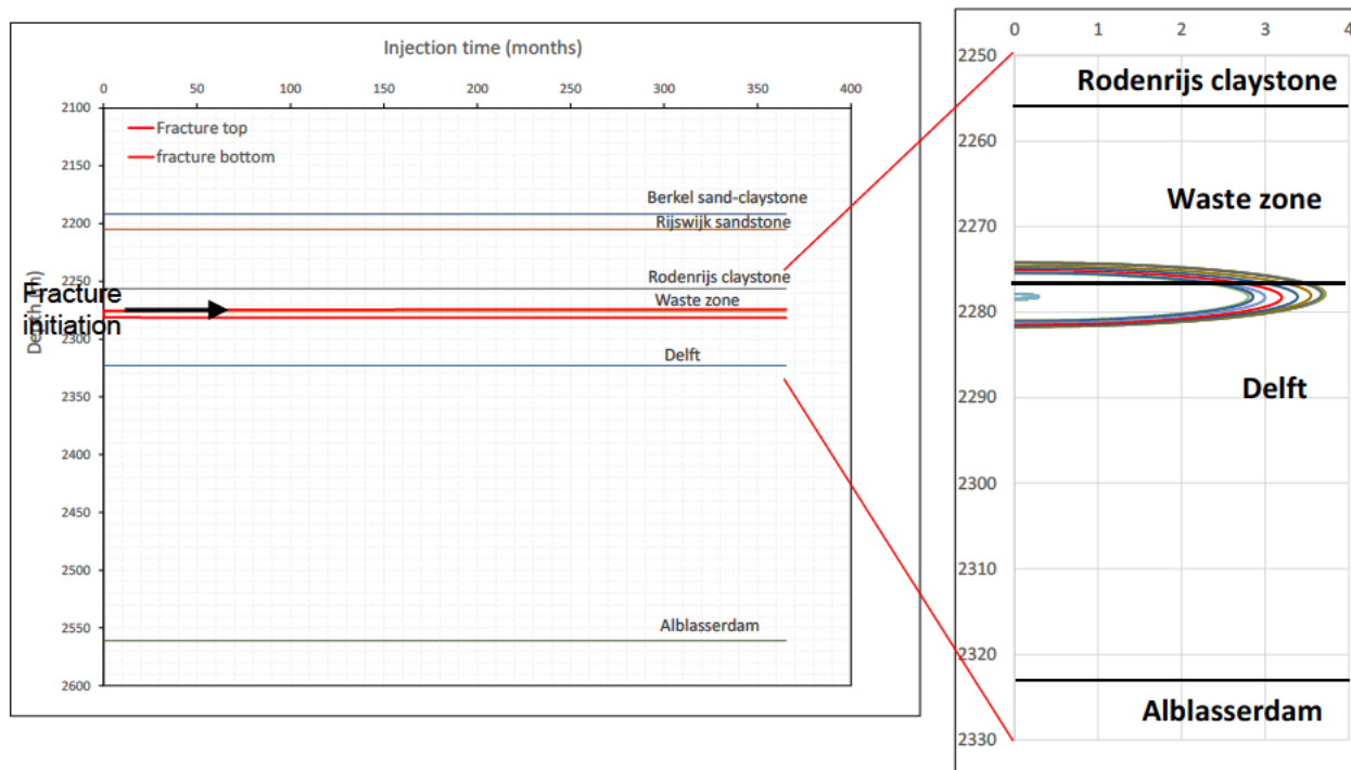
Figure 6-11: Fracture top and bottom as a function of time for base case; fracture contours for sensitivity 5. Fracture with 3.5 m radius and 2 m penetration into the waste zone. BHIP = 0.168 bar/m.
