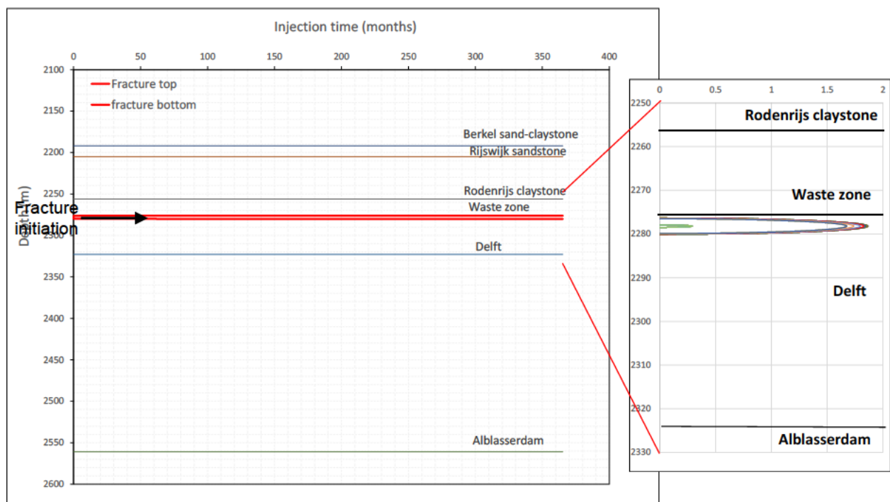
Figure 6-1: Fracture top and bottom as a function of time for base case; fracture contours for base case. Fracture remains small & entirely within the injection zone.
