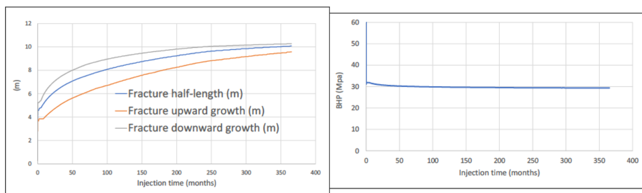
Figure 6-12: Fracture length, upward height, downward height, and Bottom Hole Injection Pressure (BHIP) for sensitivity 5. Fracture with 3.5 m radius and 2 m penetration into the waste zone. BHIP = 0.168 bar/m.
