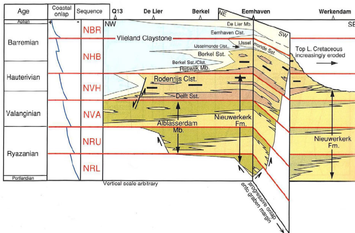
Figure 4-2: Sequence stratigraphic scheme for the Lower Cretaceous of the West Netherlands Basin based on seismic and biostratigraphic data (Den Hartog Jager, 1996). The target reservoirs of the Polanen doublet are the Cretaceous fluvial sands of the Delft Sandstone Member.
