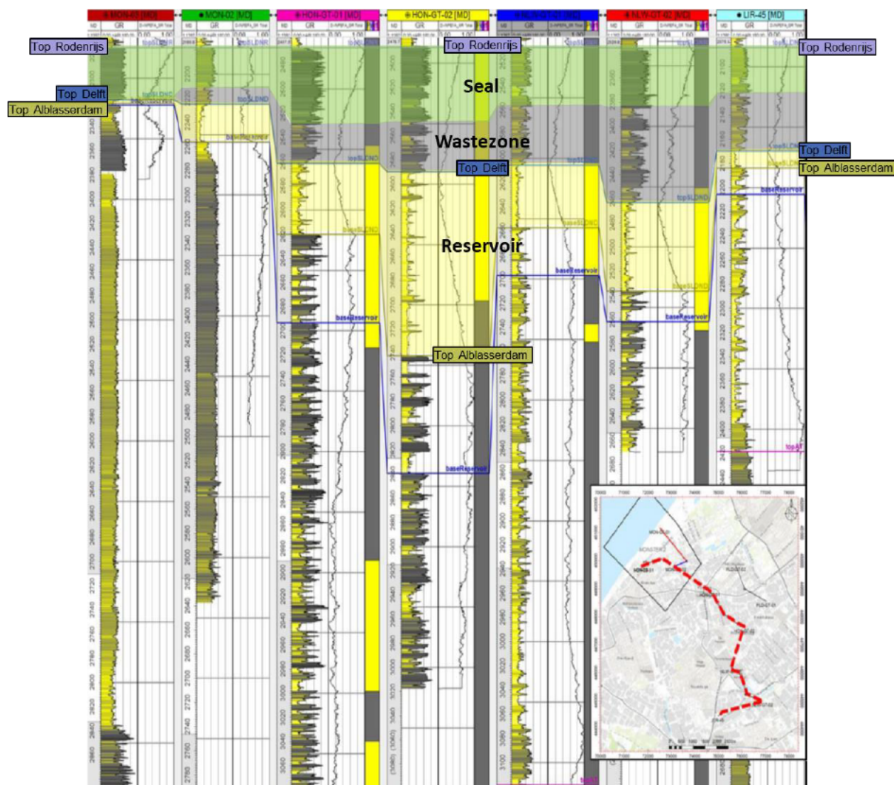
Figure 4-3: Regional correlation panel showing the gamma ray logs (non-normalised) flattened with respect to the top Rodenrijs Member. Also shown is the INPEFA log (black curve). The inlay map shows the location of the wells used, connected by the red, dashed line.
