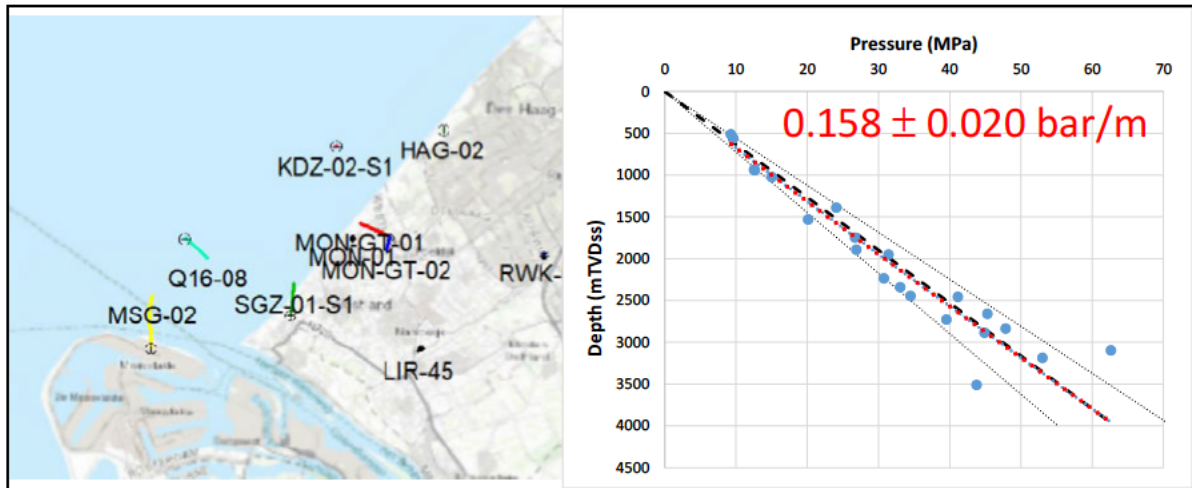
Figure 4-5: Minimum in-situ stress versus depth trend in the West Netherlands Basin area based on Formation Integrity Tests (FIT) / Leak-Off Tests from wells in the neighborhood of Polanen.
